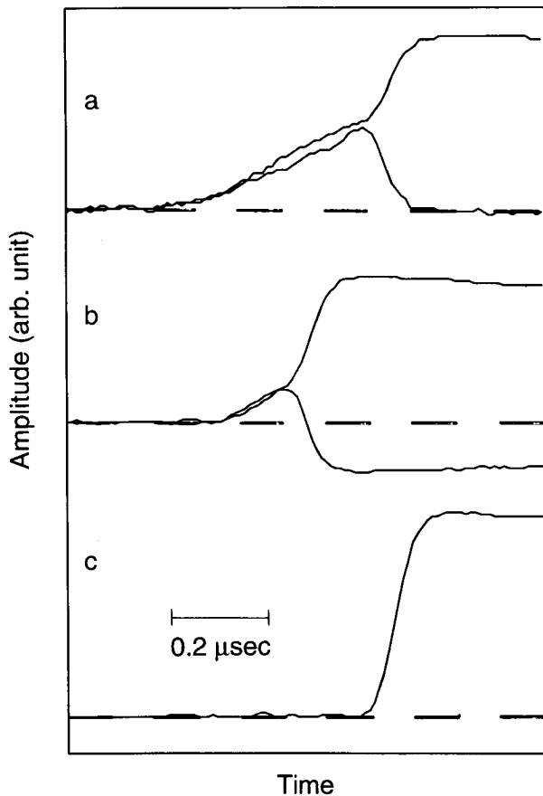
Fig. 10. (a,b) Charge signals captured simultaneously from the two grid electrodes. (c) A difference signal obtained from the output of the signal subtraction circuit. Dashed line (— — —) indicates baseline.
