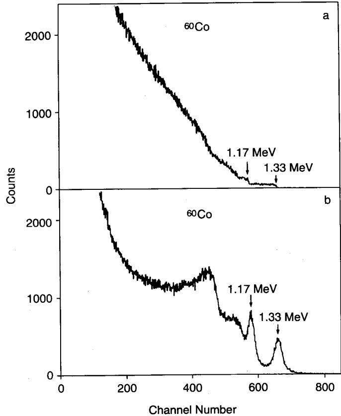
Fig. 8. ^{60}\text{Co} spectra obtained (a) with the original detector and (b) using the coplanar grid detection technique. Detector bias was 480.
