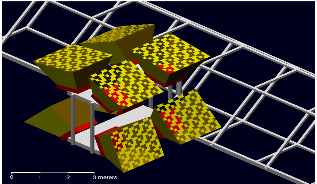
Conceptual Layout of EXIST on ISS Integrated Truss Assembly
