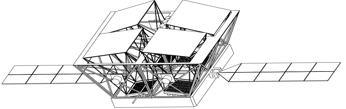
Figure 1. Layout for original EXIST concept (NMC proposal).
