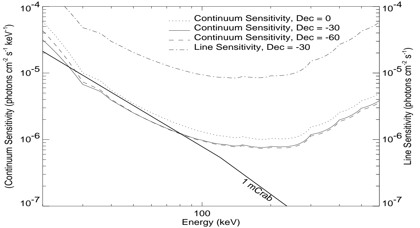
Figure 5. Estimated sensitivity for EXIST-LITE (100d flight)
