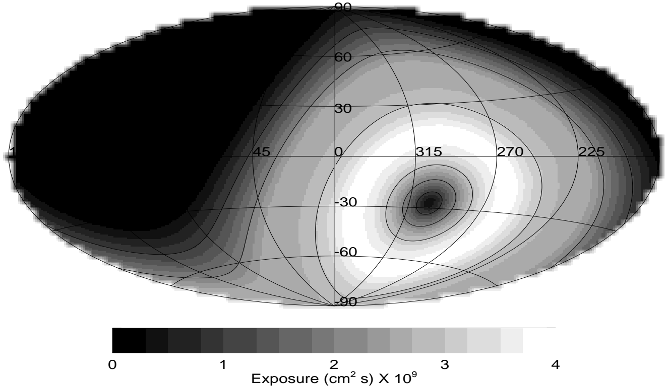
Fig. 4. Exposure time for 100d flight of EXIST-LITE.
