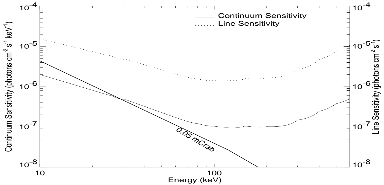
Figure 7. Exposure and sensitivity for EXIST-ISS concept.
