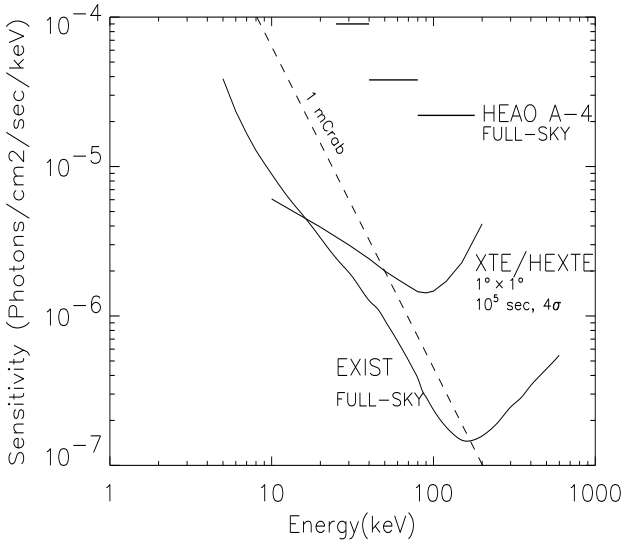
Fig 2a: EXIST-NMC Survey continuum sensitivity
