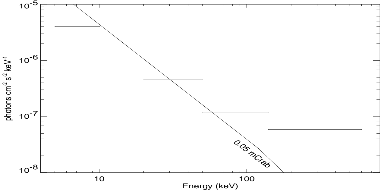
Figure 8. Continuum sensitivity ( 10^7 s survey effective exposure time) for Crab-like spectrum for EXIST-ISS concept.
