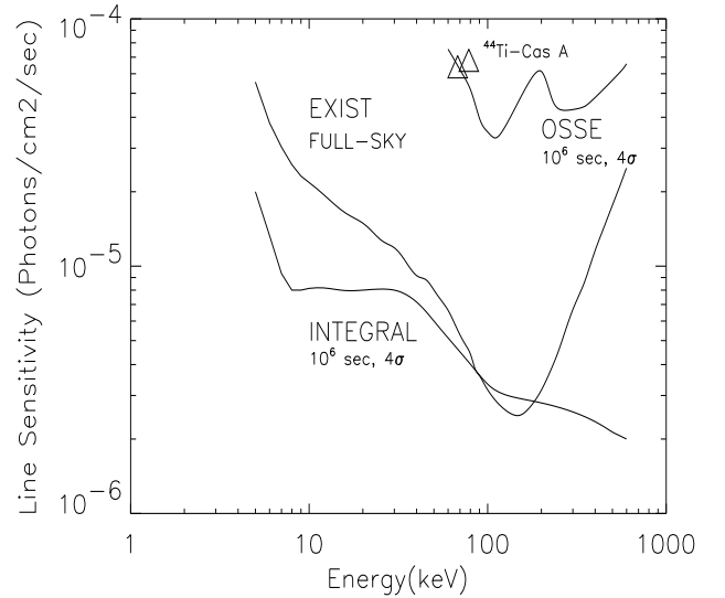
Fig 2b: EXIST-NMC Survey line sensitivity
